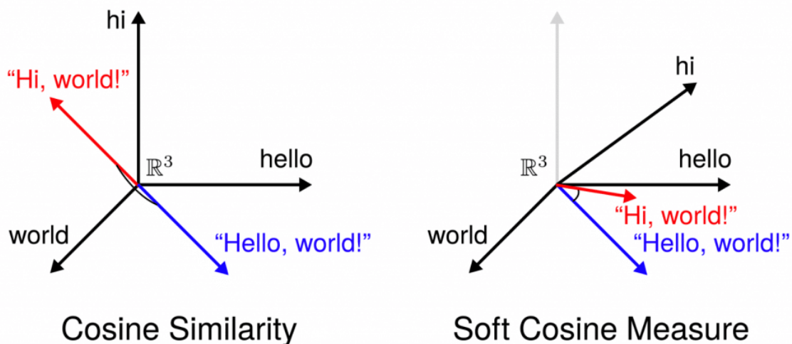
Figure 2-16. Cosine similarity and soft cosine measure
