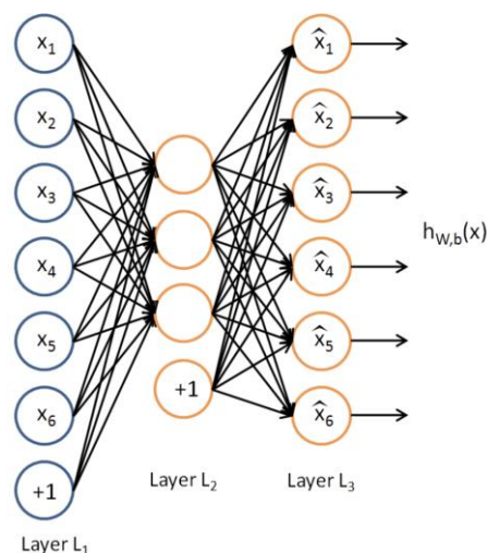
Figure 2-15. Neural network auto-encoder training
